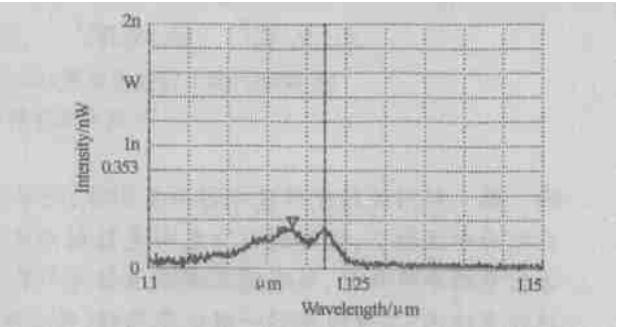
图 2 泵浦功率为 3.8 W 时测得的光谱 Fig.2 Measured spectrum with an input power of 3.8 W
